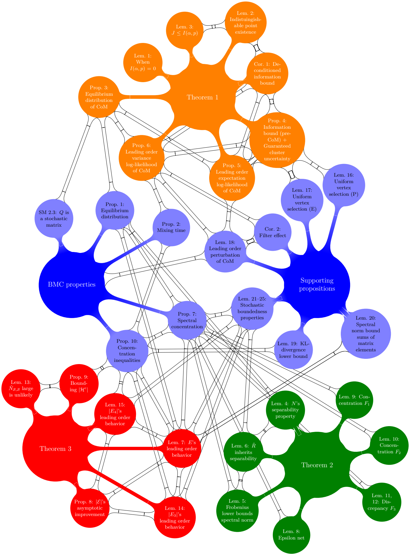
Figure 2: Mindmap after our second revision. Uncolored links correspond to the case where two results mentioned each other. CoM stands for Change-of-Measure.
